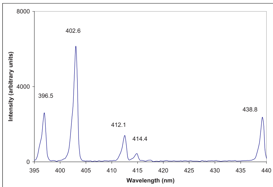
Fig. 2. A plot of part of the helium spectrum for a collection time of 5 \text{ s} .
